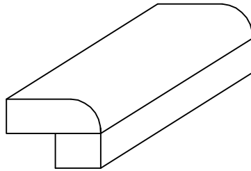
1 1/2" DEMI BULLNOSE
